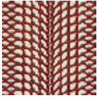
L3914_LES_EC AILLES_C526_ C534_FE
